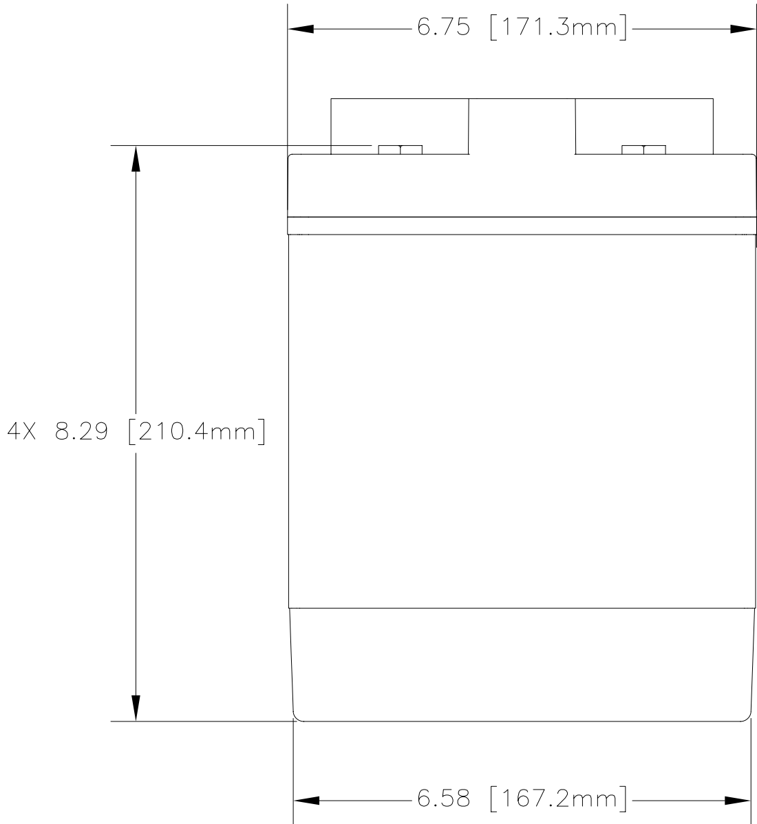
ENVELOPE DRAWING
