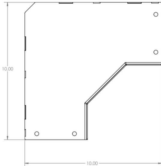
TOP/BOTTOM VIEW
