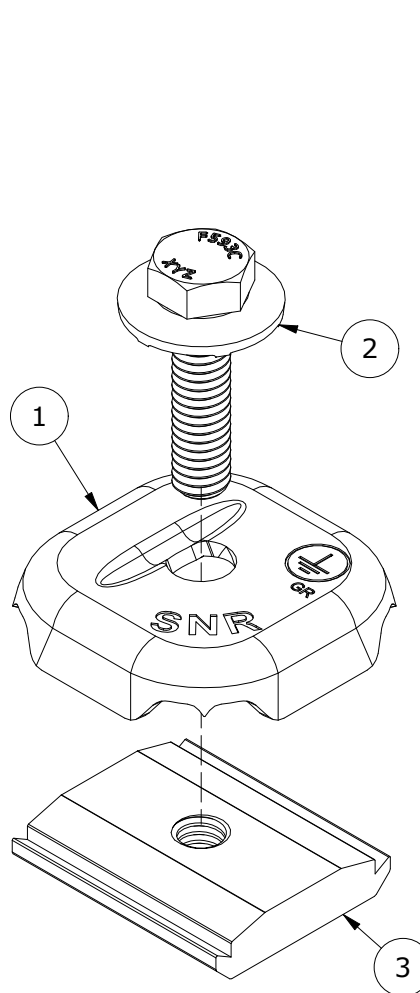
EXPLODED VIEW
