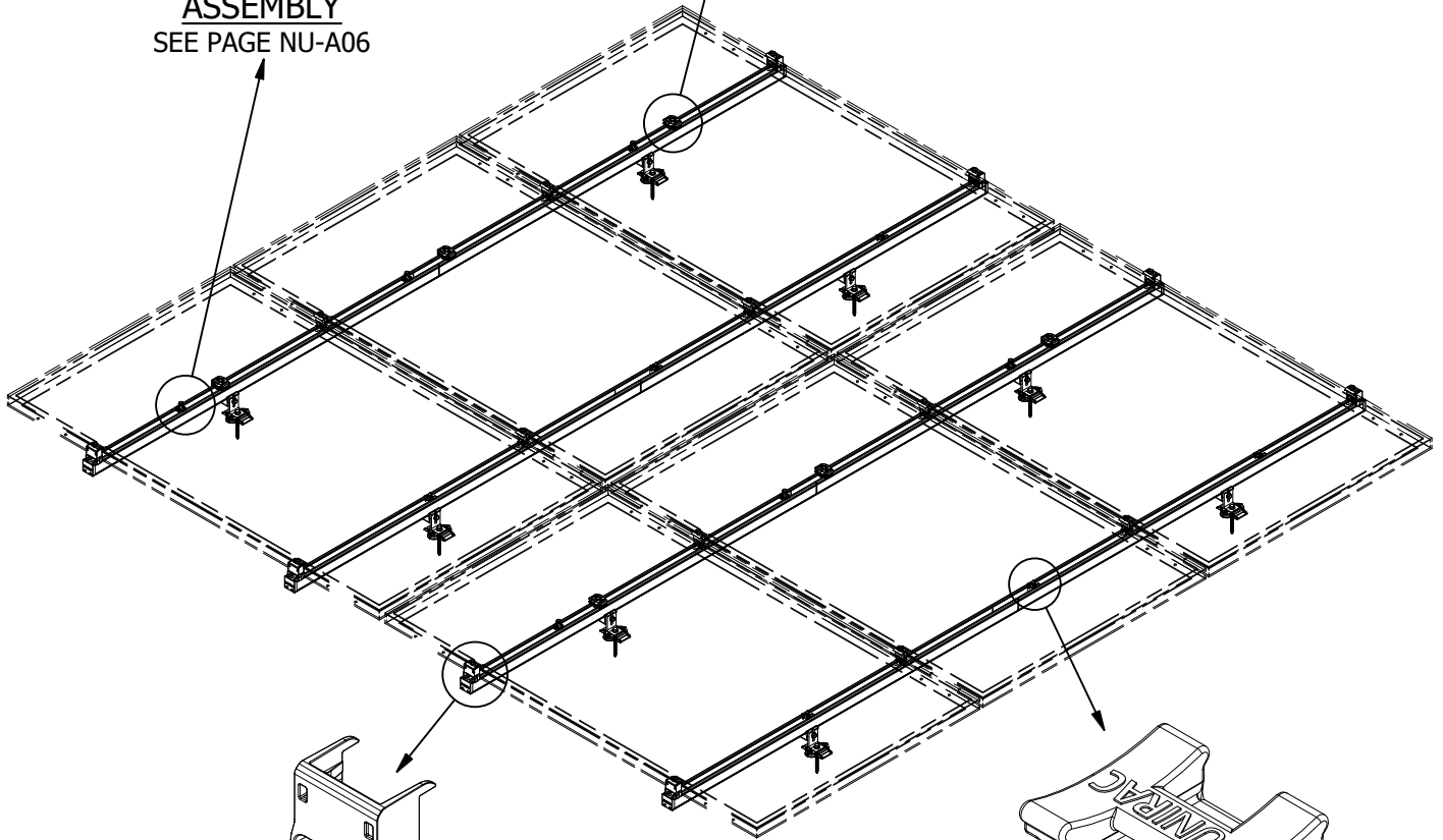
NS WIRE MGMT CLIP SEE PAGE NU-A07
