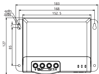
MPPT 50 A
