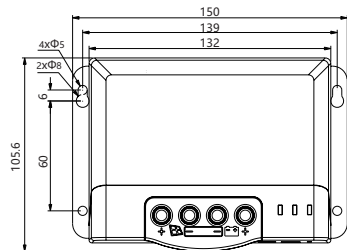
MPPT 30 A
