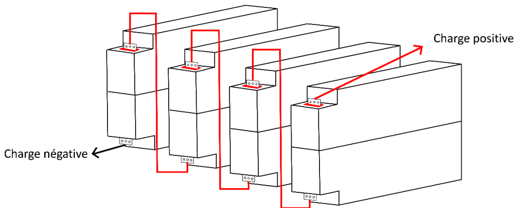
Figure 4.2: Four GC3 Batteries Connected in Series to create a 48V 270Ah Battery Ban
