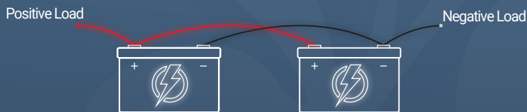
Parallel Connection 12V 540Ah Bank Increases Ah, Voltage stays the same.
