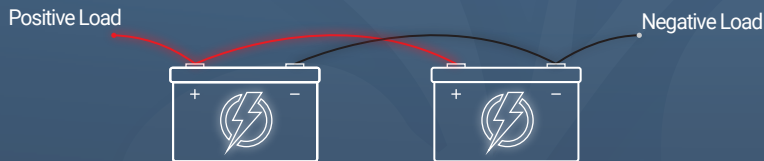
Parallel Connection 12V 540Ah Bank
