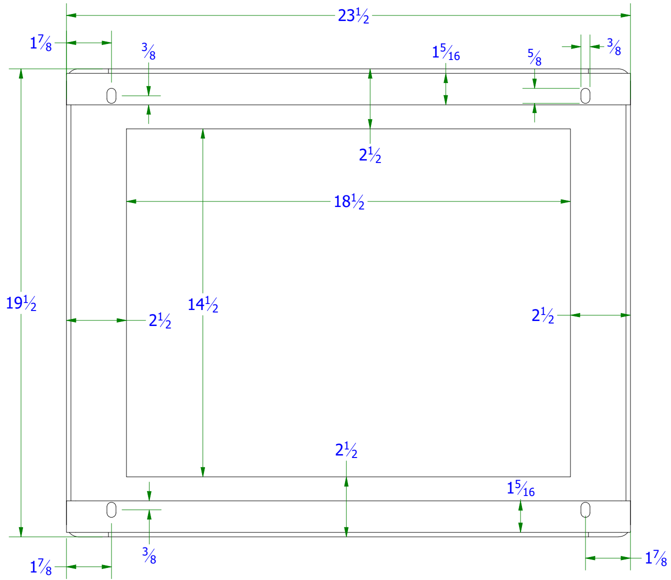
Bottom View
