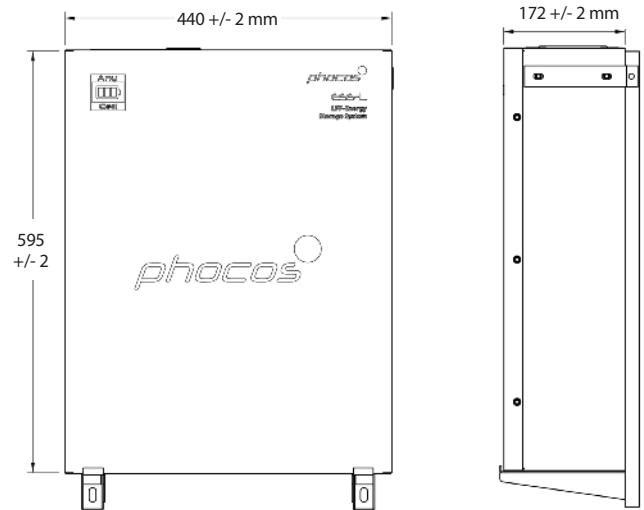
Any-Cell ESS-L-5kWh-48V
