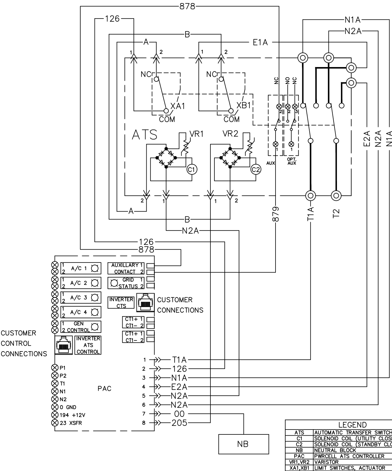
SCHEMATIC - DIAGRAM
