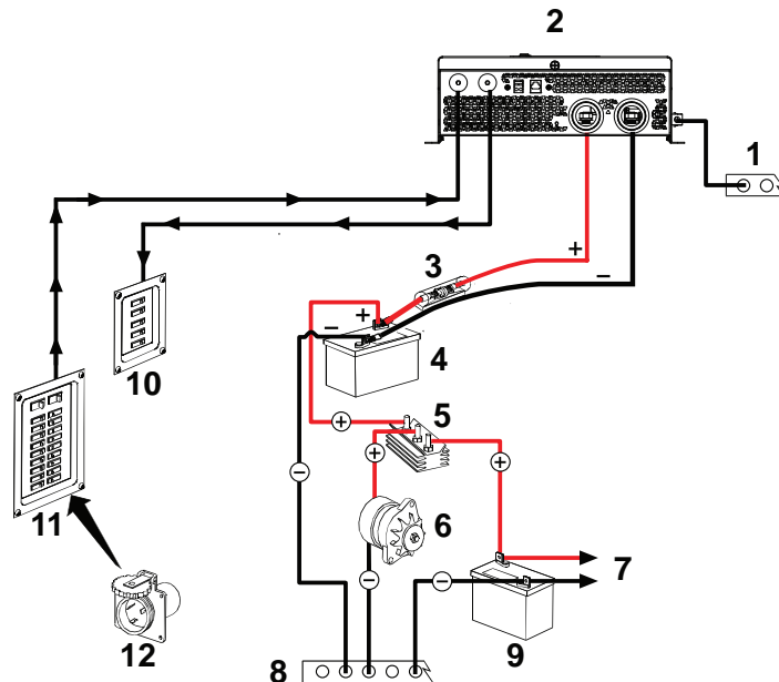
Figure 13 Installation maritimes typique
