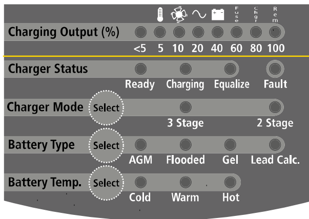
Figure 12 Onboard Display Panel
