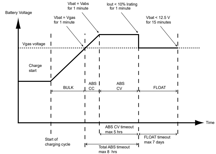
Figure 10 Three-Stage Charging Process
