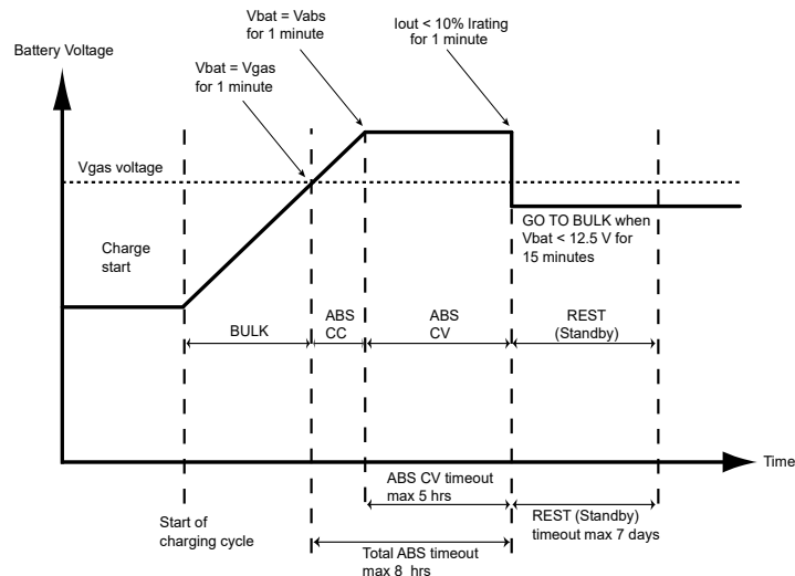
Figure 11 Two-Stage Charging Process
