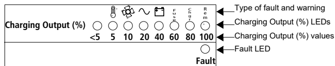
Figure 13 Charging Output (%) and Fault LEDs
