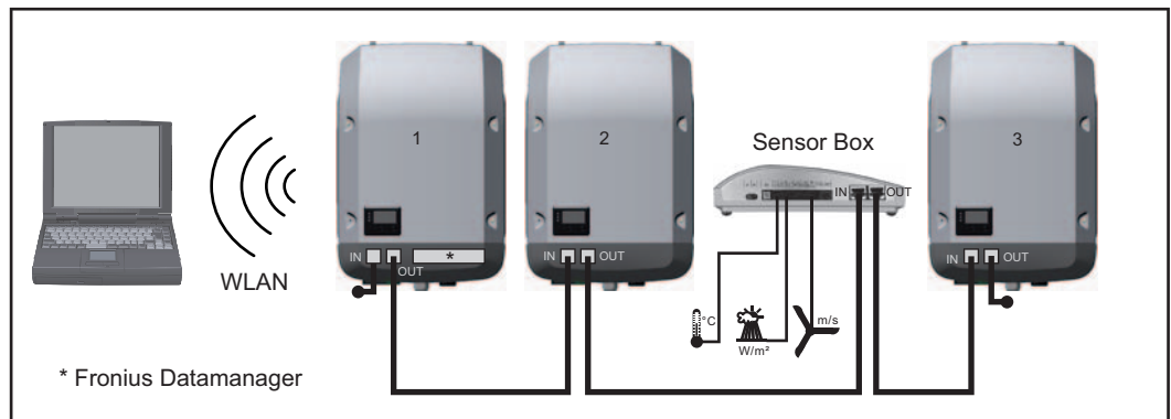
Data network with three inverters and one Fronius Sensor Box:
