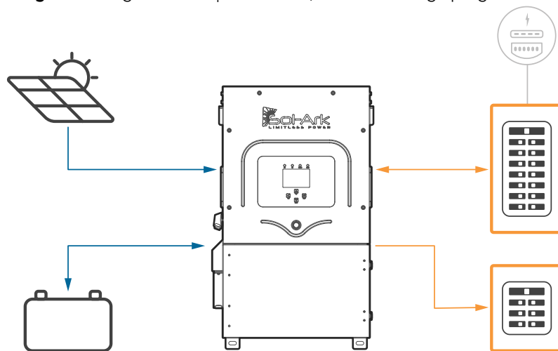
Figura 31: Limited Power to Home + TOU
