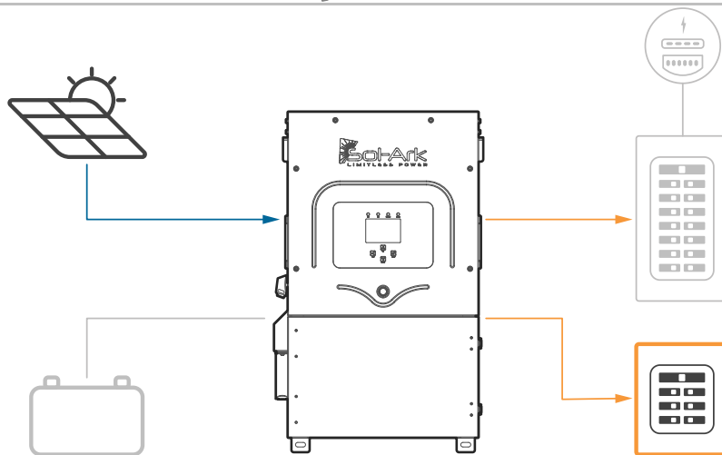
Figura 30: Limited Power to Load + Grid Sell
