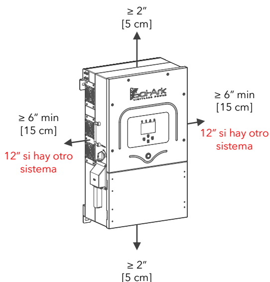
Figura 2: Unit clearances
