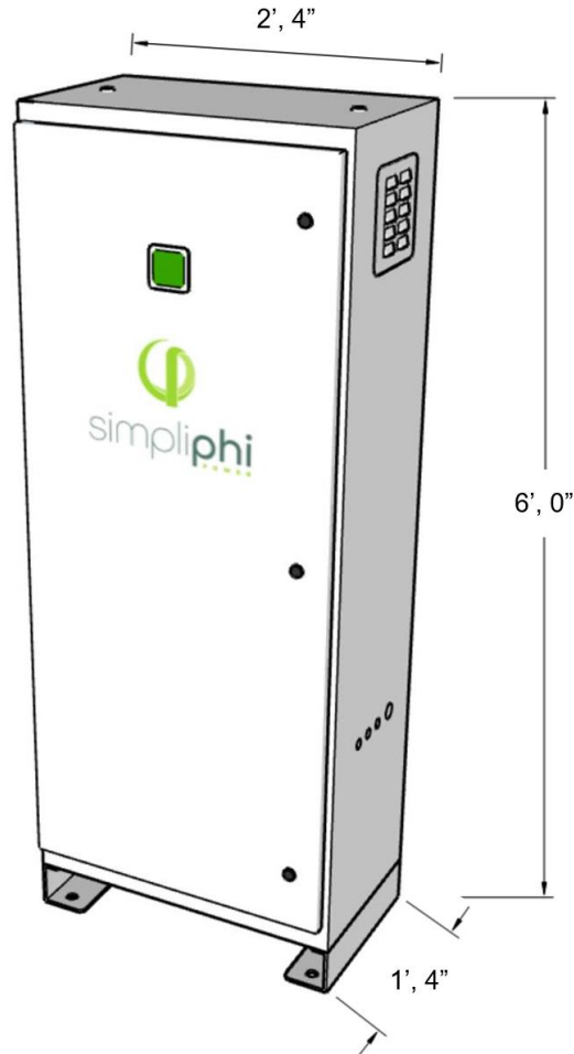
Figure 4.0 – AccESS Unit Dimensions
