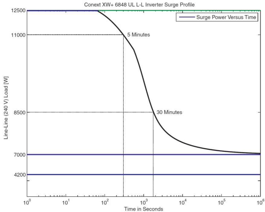
Figure 17.0 – Conext WX+ Operating Time vs 240VAC Load Graph
