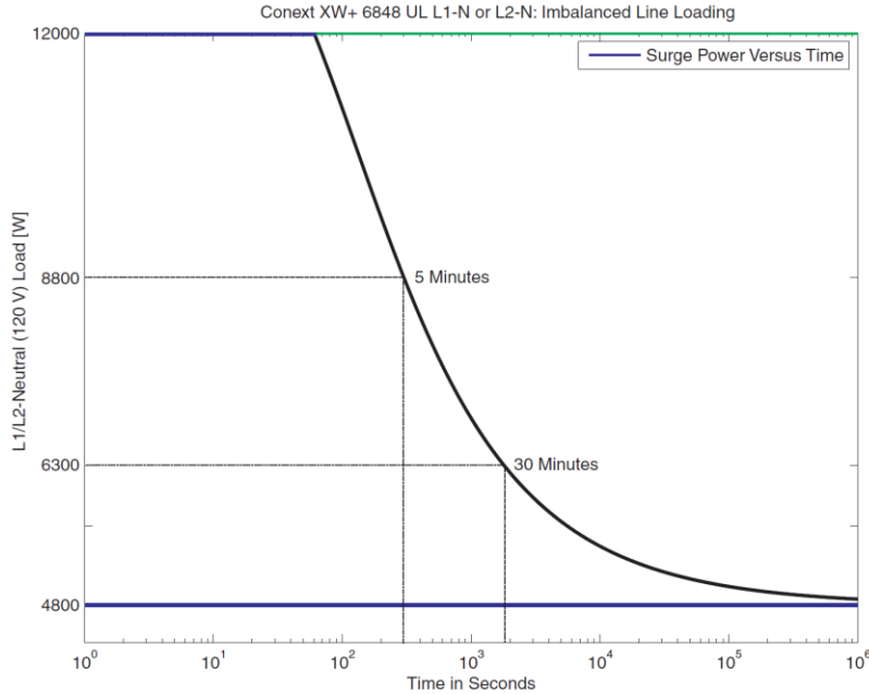
Figure 18.0 - Conext WX+ Operating Time vs 120VAC Load Graph
