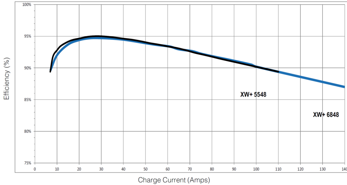
Figure 21.0 - Conext WX+ Charge Efficiency vs Current Graph
