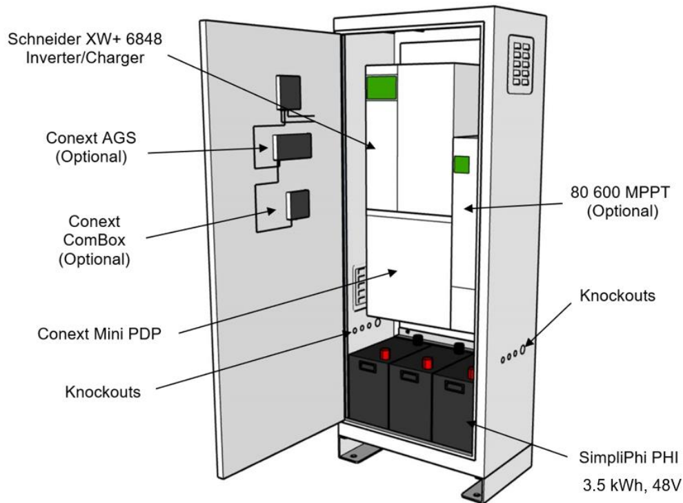
Figure 2.0 – AccESS Unit Components
