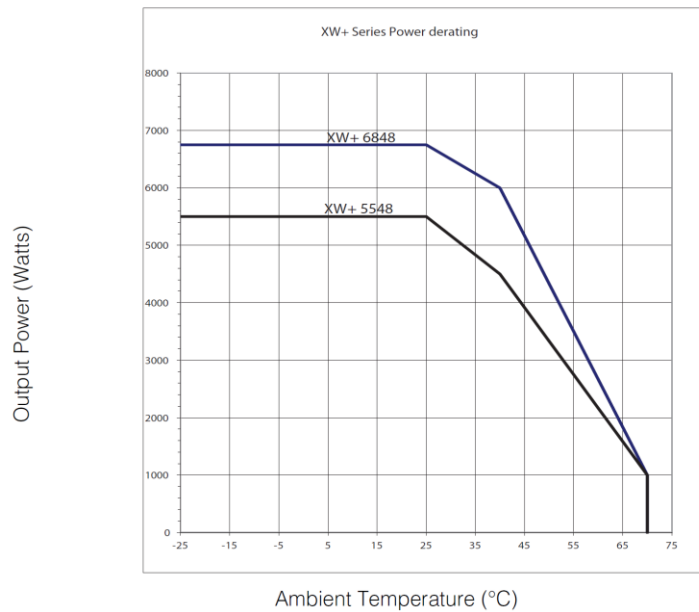
Figure 19.0 - Conext WX+ Operating Temperature vs Load Graph
