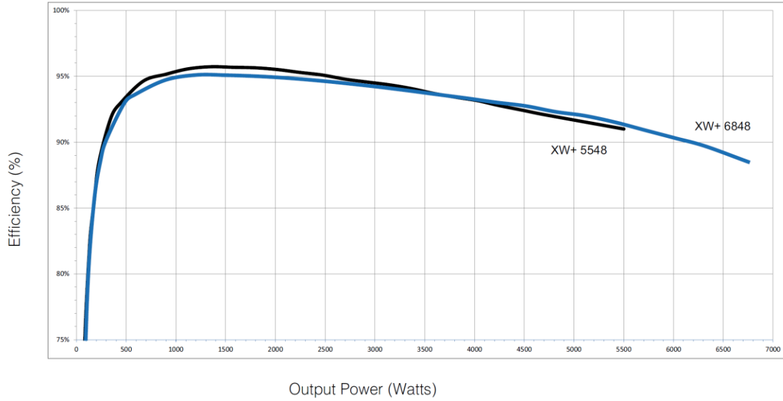
Figure 20.0 - Conext WX+ Efficiency vs Load Graph
