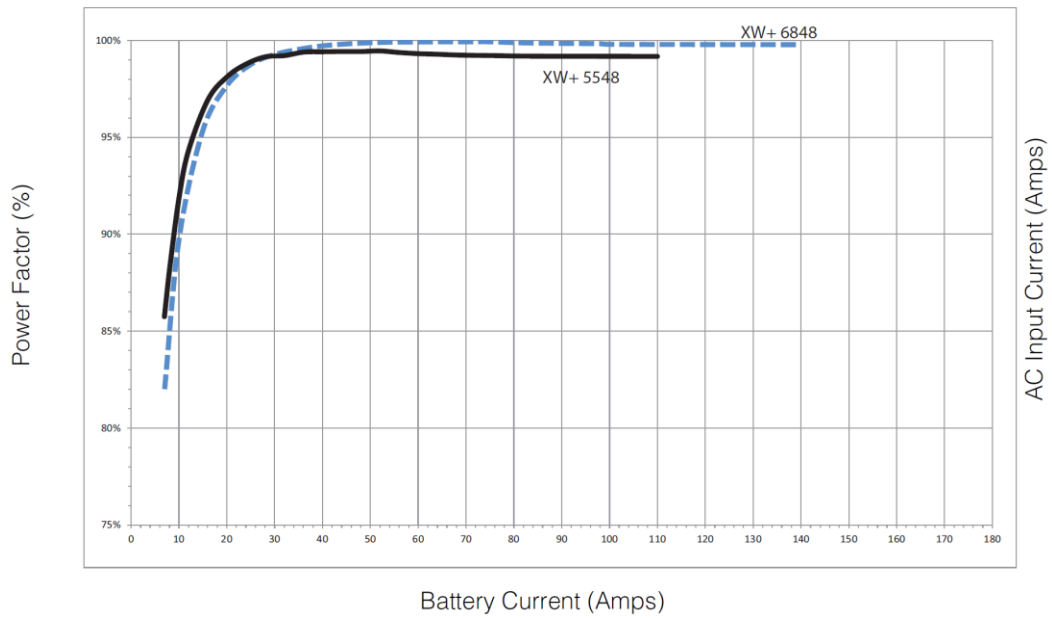
Figure 22.0 - Conex WX+ Charging Power Factor vs Current Graph
