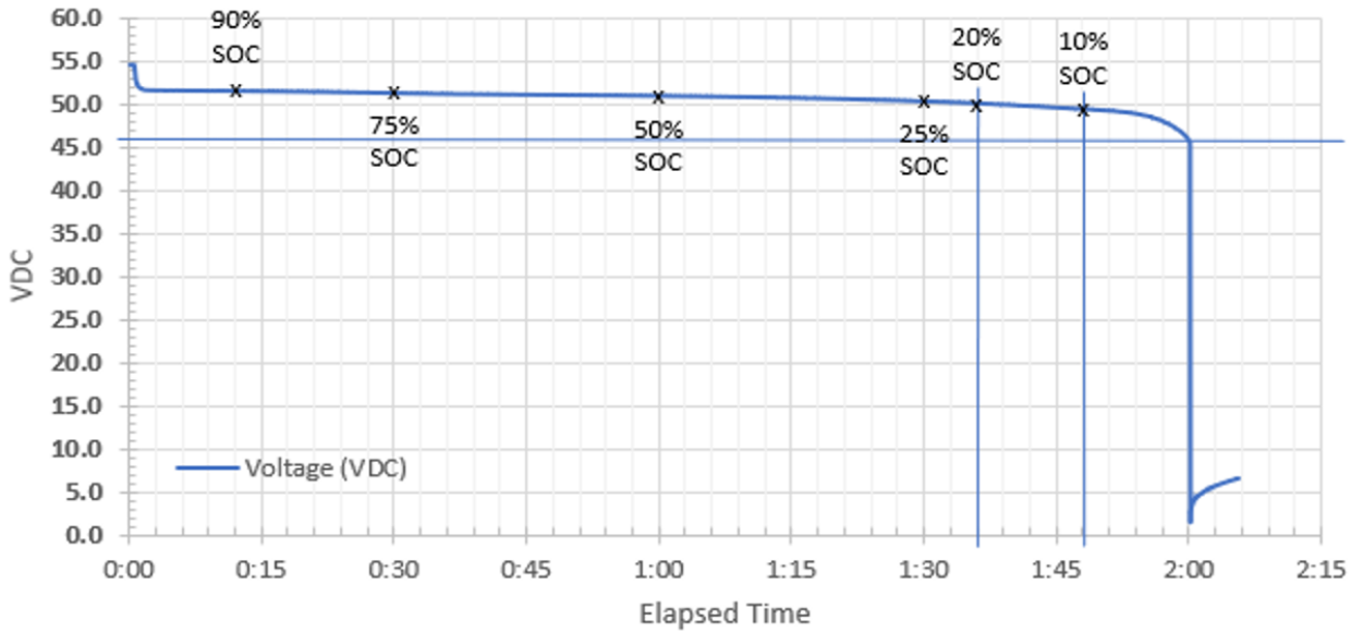
Figure 16.0 – PHI 3.5 C/2 Discharge Curve (typical)
