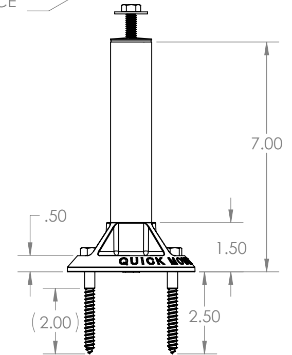
QBASE (ITEM 2) AND POST (ITEM 7)
