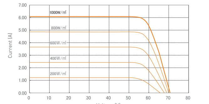
Reference data for model: VBHN330SA17 (Cell temperature: 25°C)
