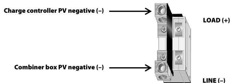
Figure 8 Positive-Grounded RTB
