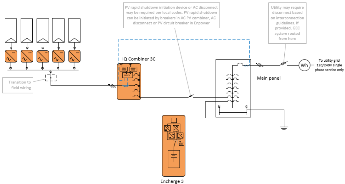
Figure 9: Grid interactive Encharge storage system installation with no backup on IQ6/7 microinverter sites
