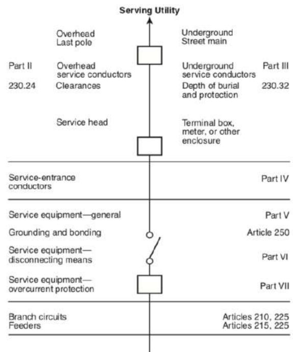
Figure 12: NEC 2017 Figure 203.1 Services © NFPA
