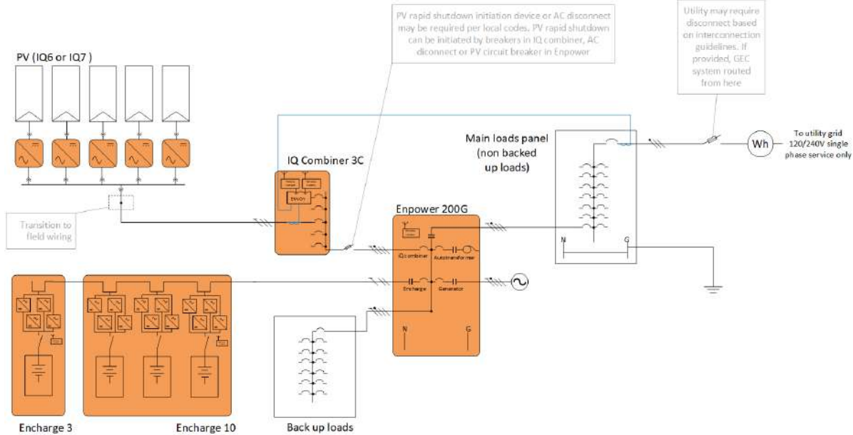
Figure 4: Always-On Ensemble technology system with partial home (subpanel) backup for IQ-Series microinverters. Enpower is installed on the load side of the main load panel with select loads backed up in a backup subpanel.
