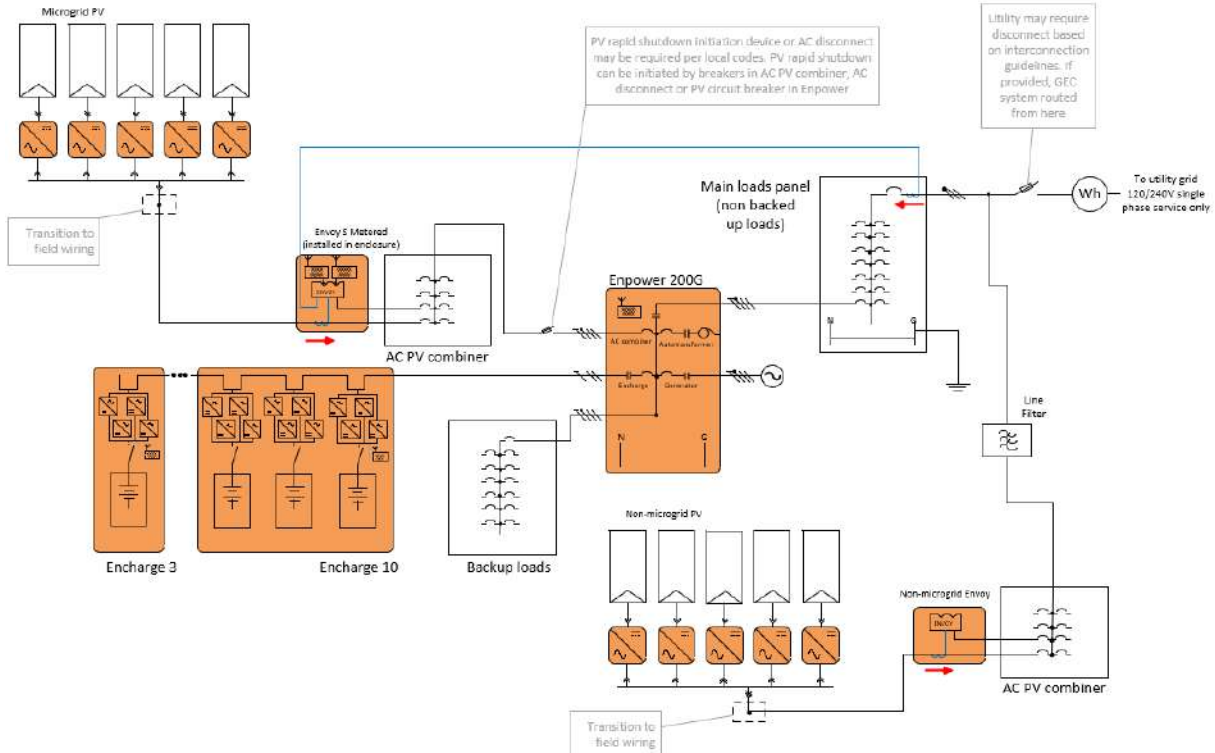
Figure 8: M-Series "split" PV system that does NOT require an additional set of Consumption CTs
