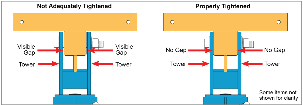
Tighten Pivot Bolt closing any visible gaps between the Strongback and the Mounting Sleeve Towers. Torque to 330-350 ft.-lbs.
