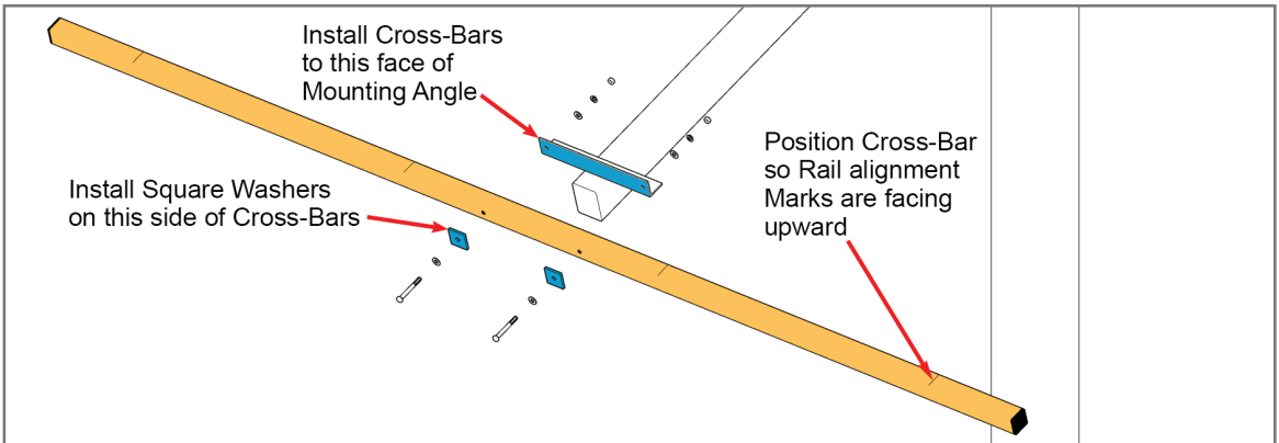
Install the three Cross-Bars with 3/8" x 3-1/4" Hex Bolt, Square Washer, Flat Washers, Lock Washer and Hex Nut. Tighten and torque to 30-32 ft.-lbs.
