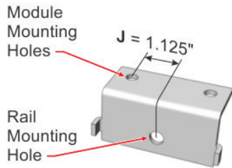
"J" Factor of Double Hole Slide Plate
