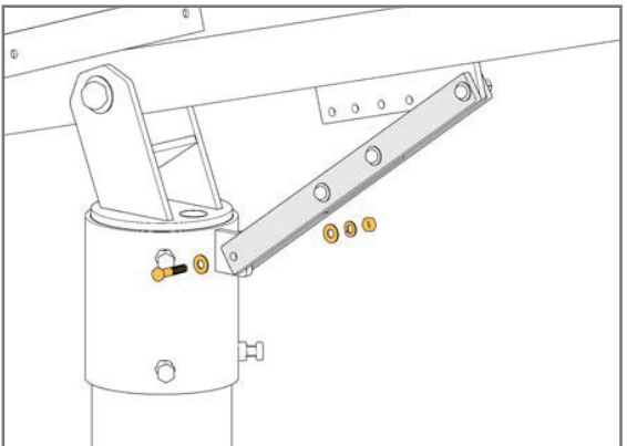
Torque Support Bar hardware at 32-34 ft.-lbs.
