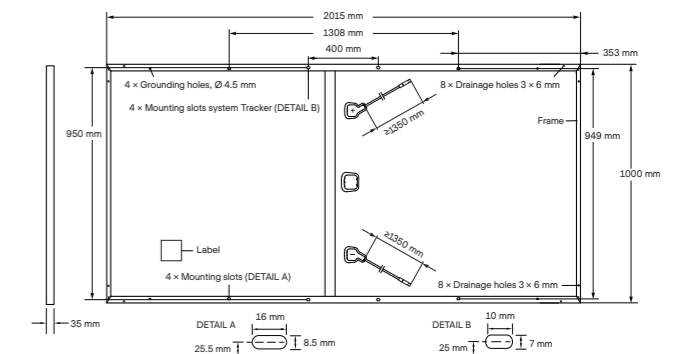
Fig. 2: External dimensions (in mm) and components for Q.PEAK DUO L-G5.1, Q.PEAK DUO L-G5.2, Q.PLUS DUO L-G5.1 and Q.PLUS DUO L-G5.2
