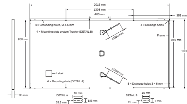
Fig. 1: External dimensions (in mm) and components for Q.PEAK DUO L-G5, Q.PEAK DUO L-G5.3, Q.PLUS DUO L-G5 and Q.PLUS DUO L-G5.3
