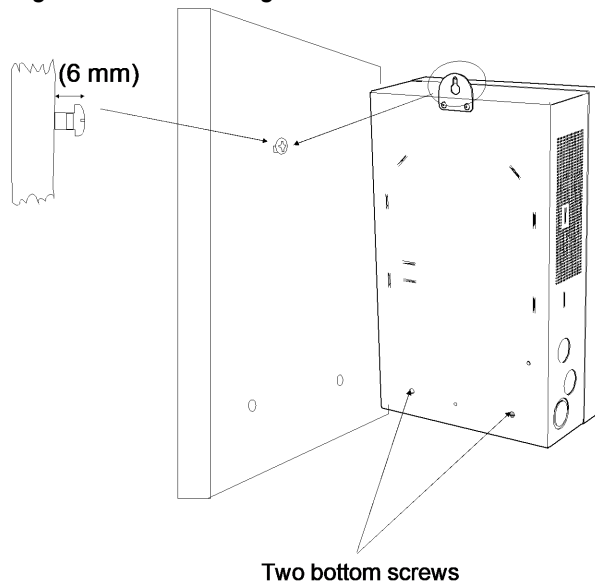
Figure 6 Wall mounting
