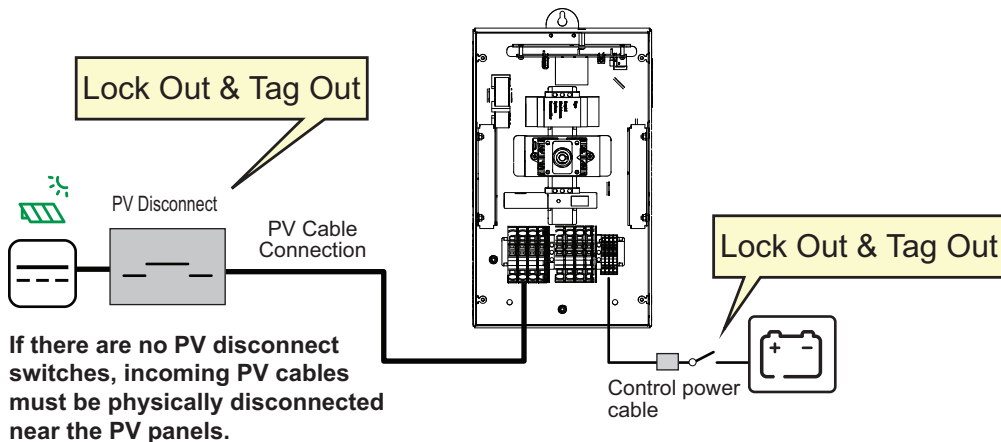
Figure 2 LOTO
