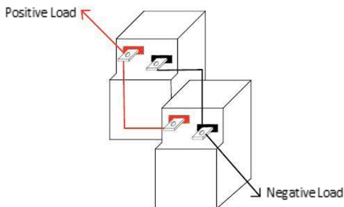
Figure 3: Two BBGC2 Batteries connected in Parallel to create a 12V 200Ah Battery Bank
