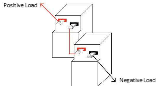
Figure 4: Two BBGC2 Batteries Connected in Series to create a 24V 100Ah Battery Bank
