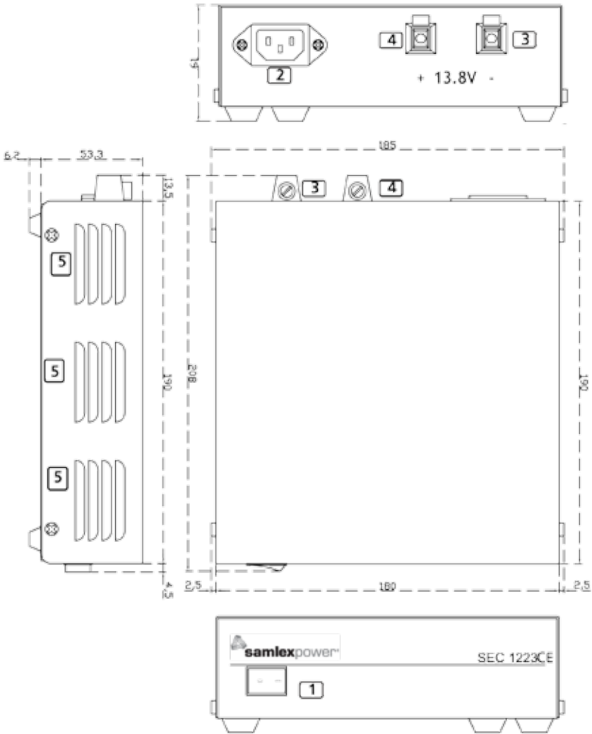
Figure 2.2 Layout & Dimensions - SEC-1223CE
