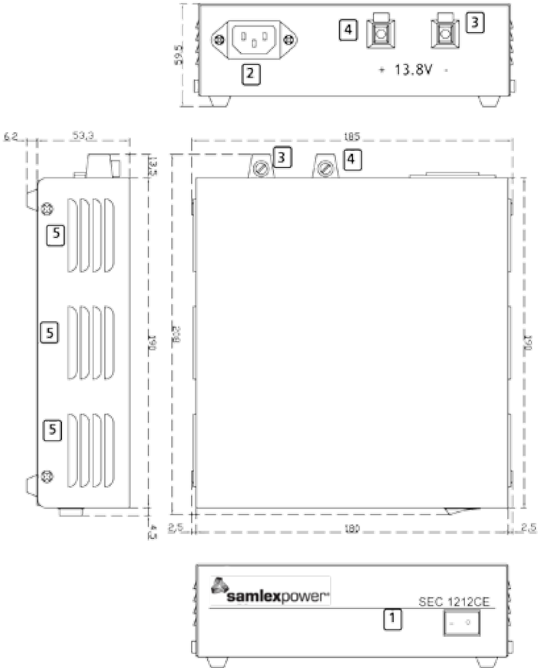
Figure 2.1 Layout & Dimensions - SEC-1212CE
